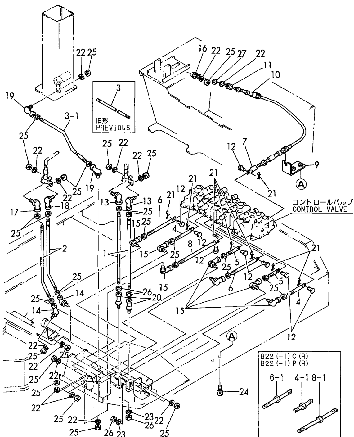
Fig. 23 操縦装置 (ロッド) CONTROL EQUIPMENT (ROD)
