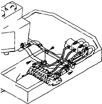
Fig.51 油圧配管 (走行) HYD. OIL PIPING (TRAVEL)
