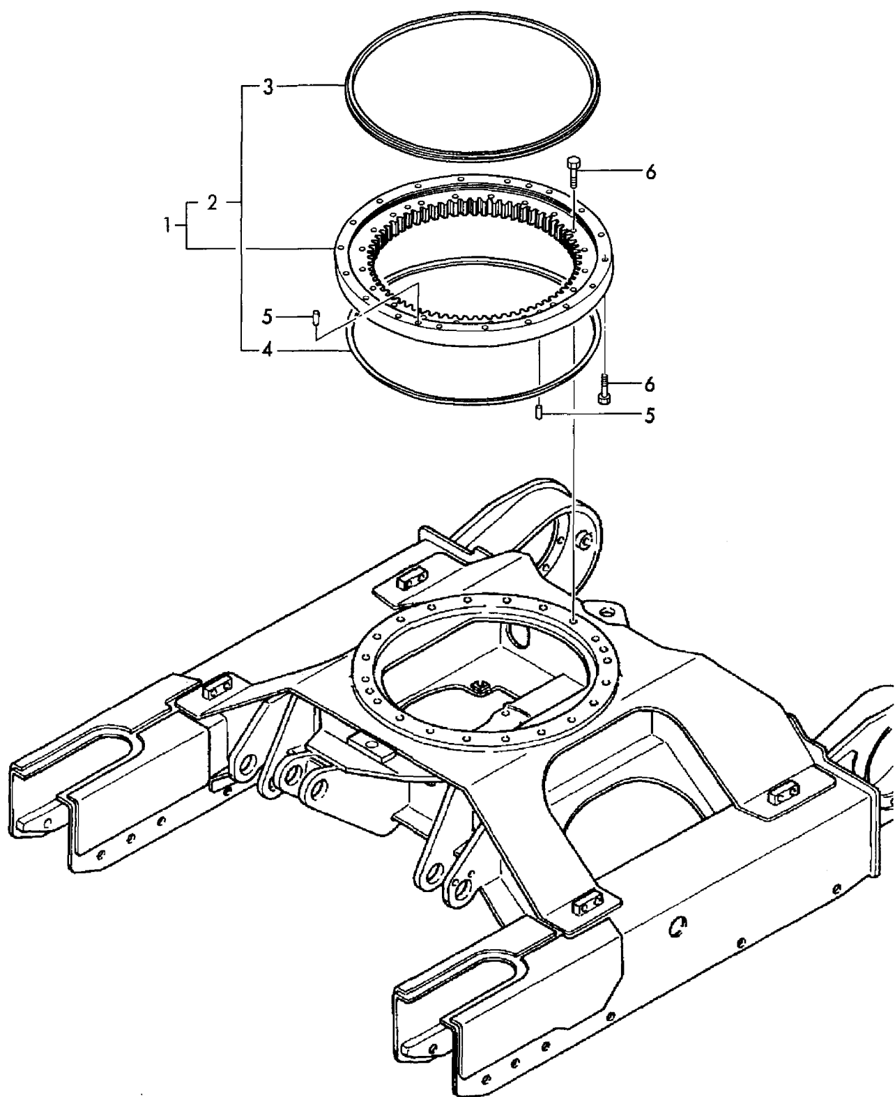
Fig. 26 旋回駆動装置 TURNING DRIVING GEARS
