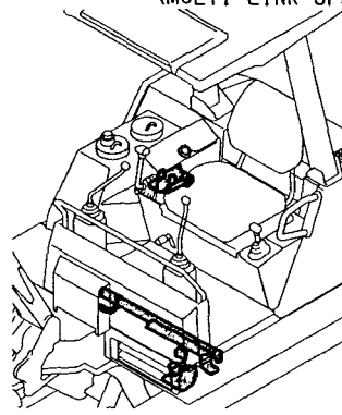
Fig.23 操縦装置 (ロッド) CONTROL EQUIPMENT (ROD)
